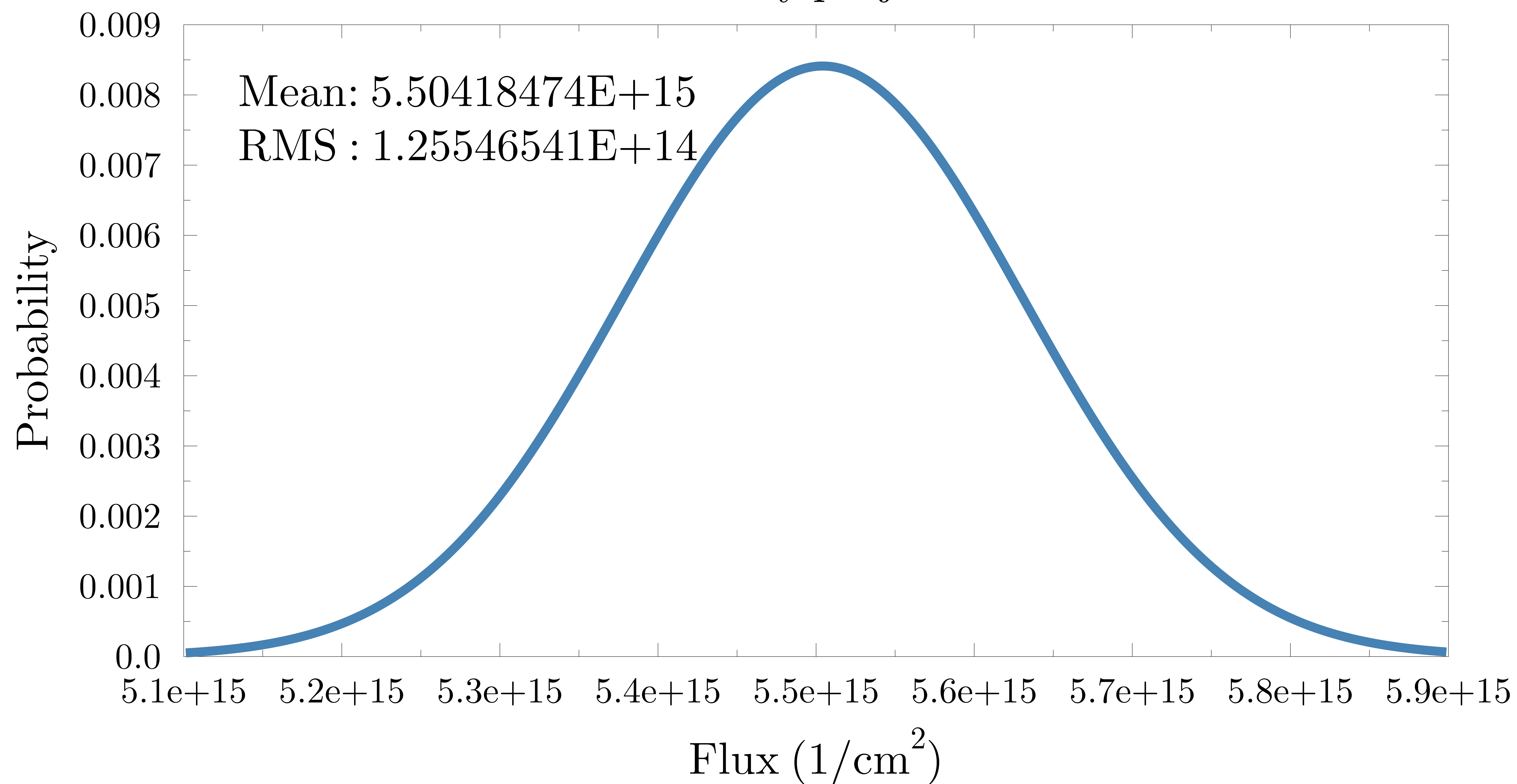
Probability projection-x
