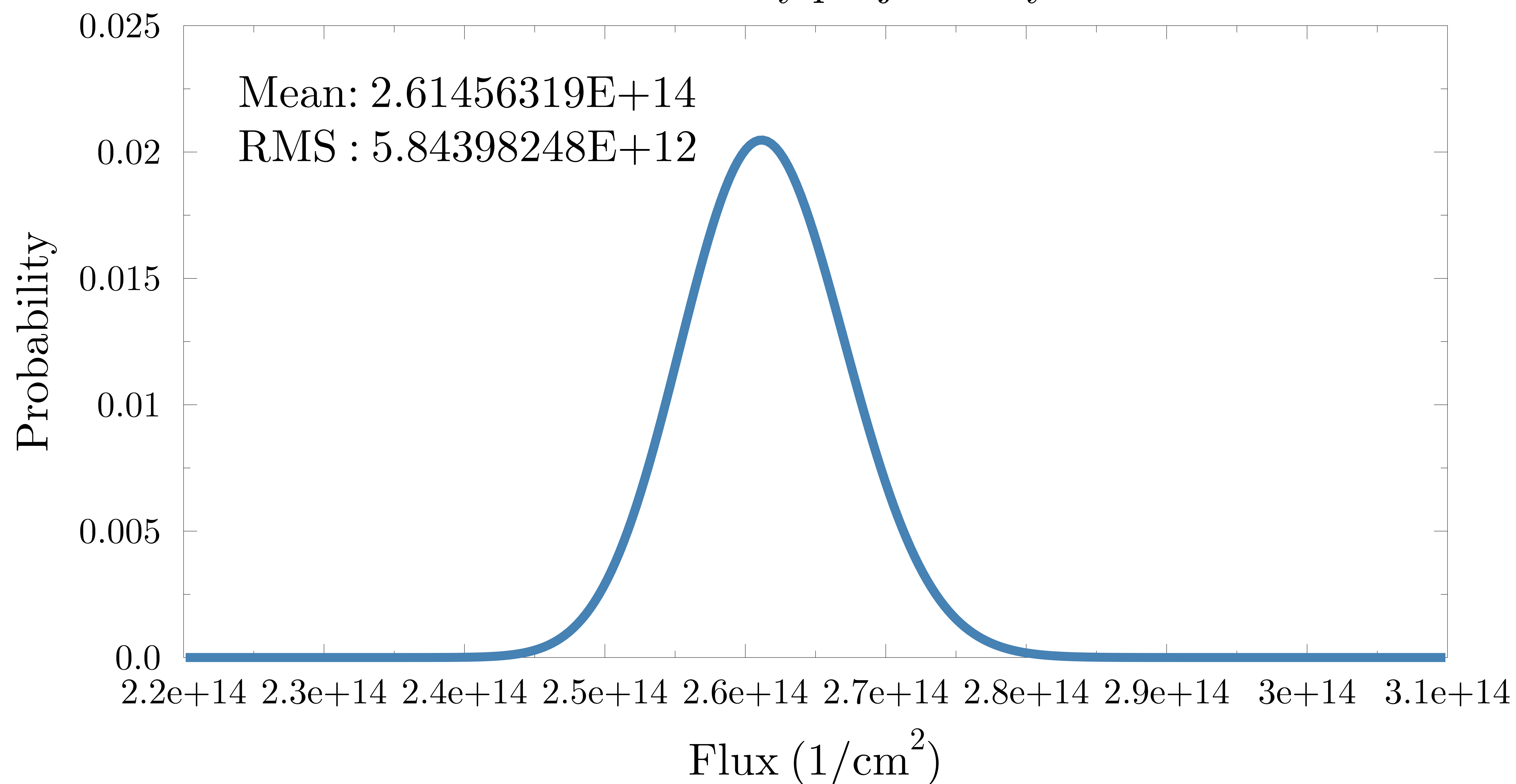
Probability projection-y
